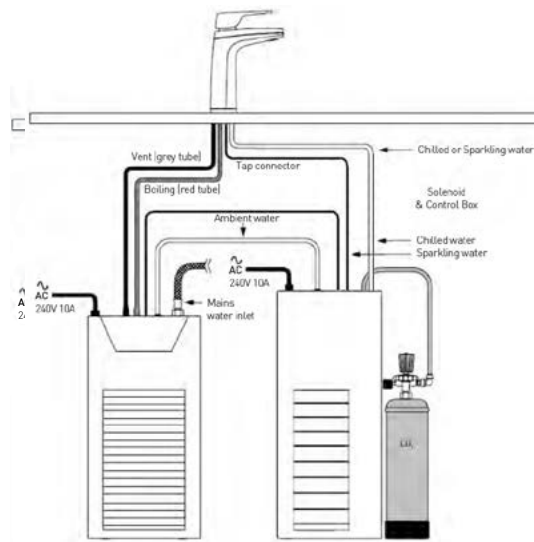
Preferred Eco & Quadra Sparkling Installation layout
