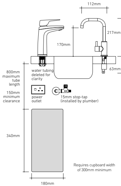
Preferred Alpine installation layout
